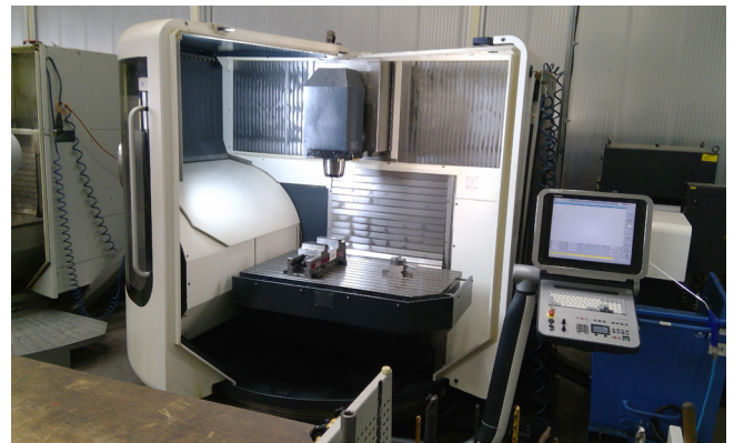
Pos. 61 1 CNC Bohr- und Fräsmaschine Deckel Maho DMU 80 monoBLOCK 1 CNC Milling/drilling machine Deckel Maho DMU 80 monoBLOCK
