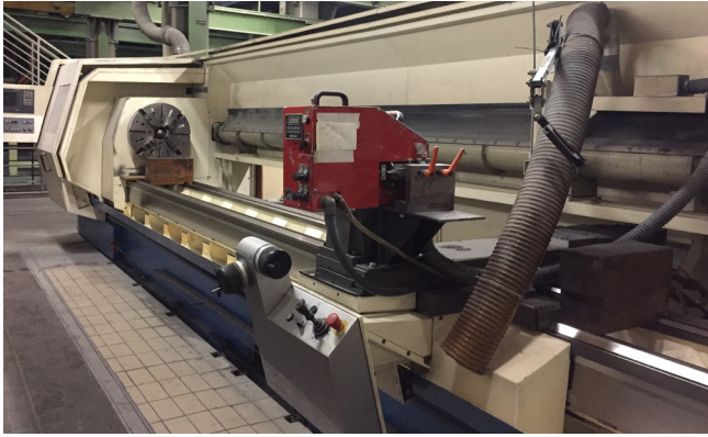
Pos. 41 1 CNC-Drehmaschine VDF Boehring DUS 1000 ti, Bj. 2001 1 CNC turning lathe VDF Boehring DUS 1000 ti, YOM 2001
